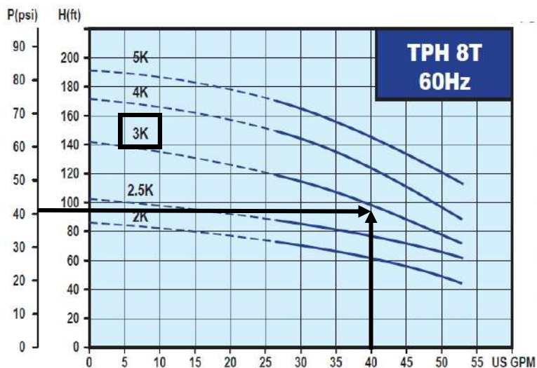
Performance curve for each pump
